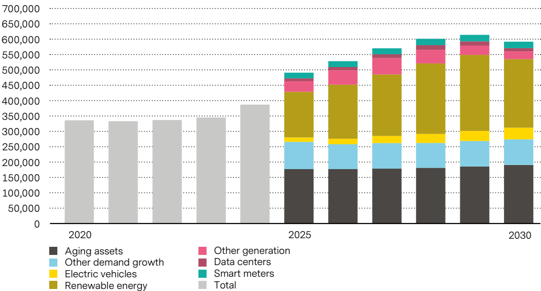
Figure 2: Global annual grid investment by main driver
